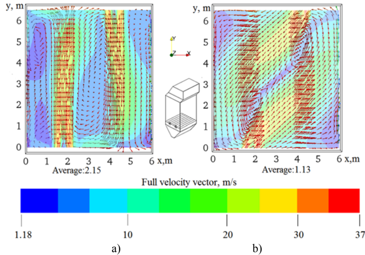
Figure 2 - Distribution of the full velocity vector in the region of the burner ( z = 4.0 m) combustion chamber of the boiler BKZ-75 in emergency mode :
