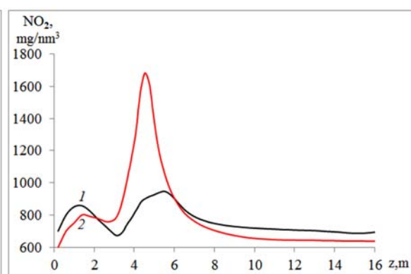
Figure 6 - Distribution the concentration of nitrogen dioxide NO 2 at the exit of the combustion chamber the boiler BKZ-75 emergency mode :
