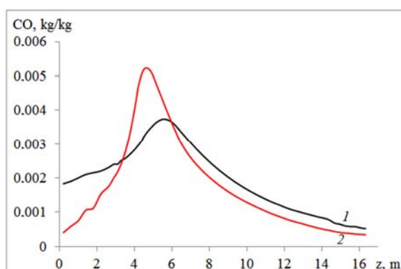
Figure 5 - Distribution the concentration of carbon monoxide CO at the exit of the combustion chamber the boiler BKZ-75 emergency mode :
