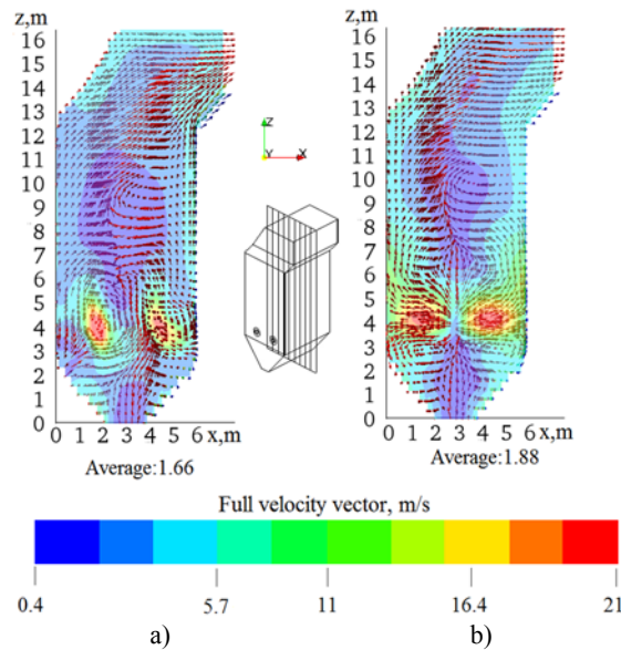
Figure 3 - Distribution of the full velocity vector in the central longitudinal section ( y=3.3 ) of the combustion chamber of the boiler BKZ-75 in emergency mode :
