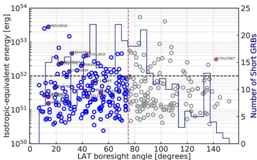
Figure 2 - Distribution of 363 short GRBs by LAT boresight angle and isotropic-equivalent energy calculated under assumption of common z=1 . Vertical dashed lines indicates \theta=75 degrees threshold angle for LAT instrument, horizontal dashed line indicates E_{iso}=1e52 erg energy
